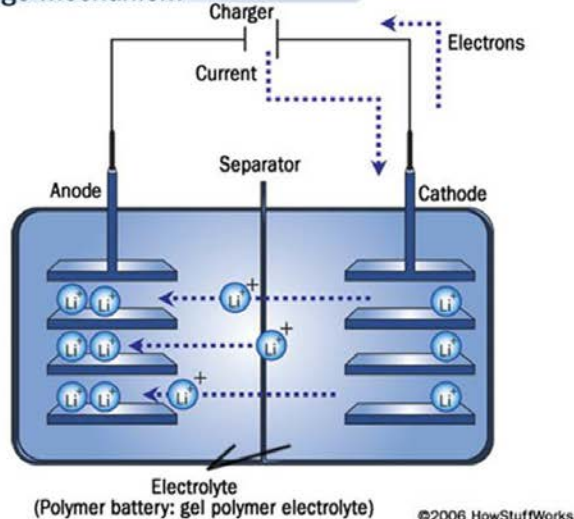
Lithium-ion rechargeable battery Charge mechanism
